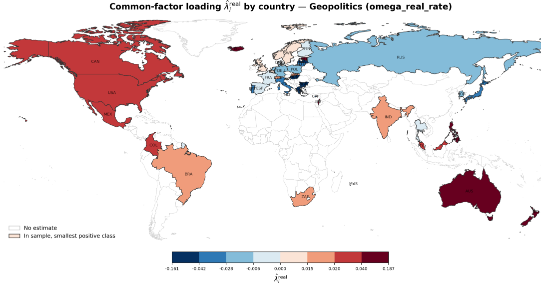
Figure 6: Spatial Distribution of Country-Specific Factor Loadings
